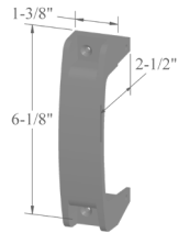
Gate Handle S3 LL3GH
